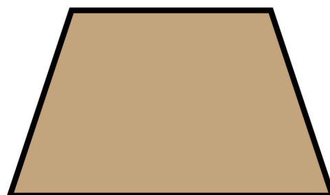
TRAPES
