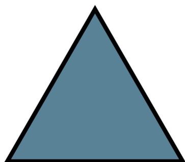
LIKESIDET TREKANT
