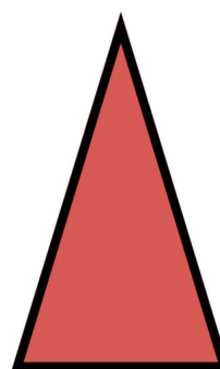
LIKEBEINT TREKANT
